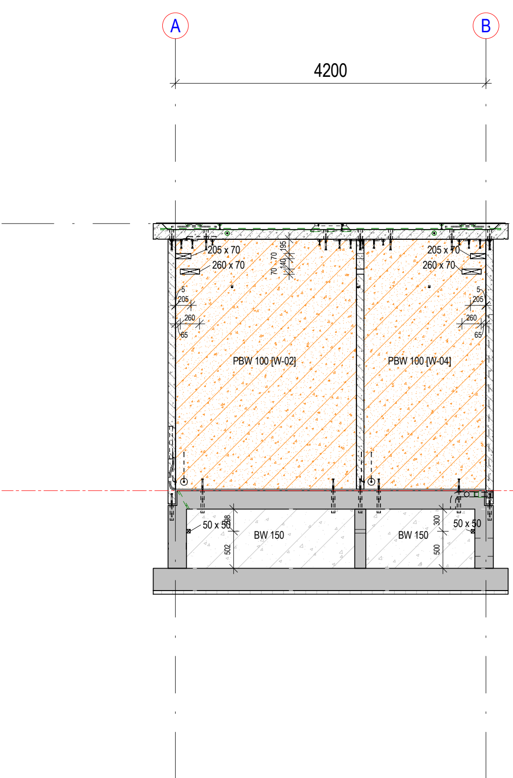
wand as 2-3
