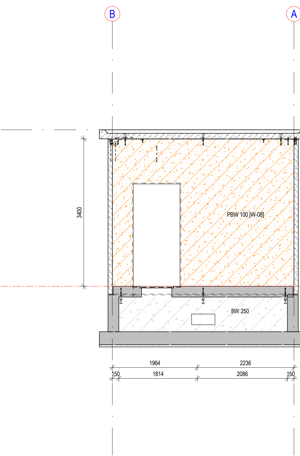
wand as 4
